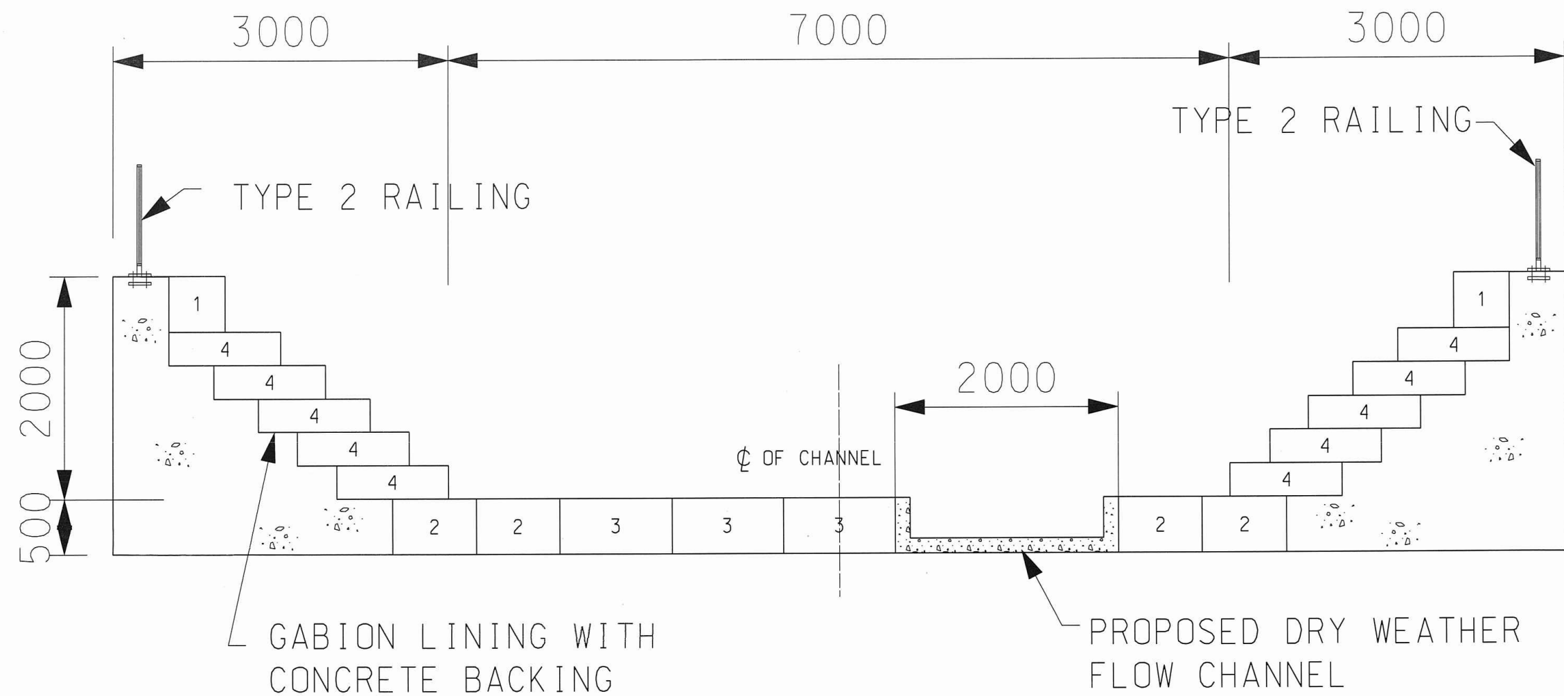
TYPICAL CROSS SECTION OF TRAPEZOIDAL CHANNEL (WITH DRY WEATHER FLOW CHANNEL AND GABION LINING) N. T. S.
